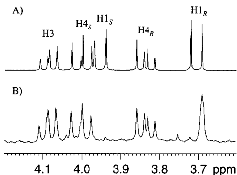
Figure 2. Partial ^1\text{H} NMR spectrum of 2- C -methylerythritol bisacetone. (A) Unlabeled standard. (B) Monodeuterated product derived from enzymatic reaction.
