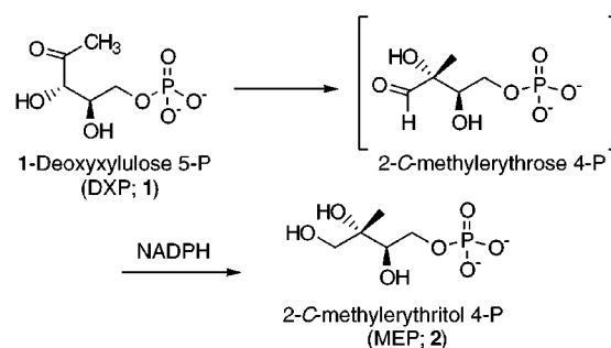
Figure 1. Conversion of DXP to MEP by DXP isomeroreductase.
