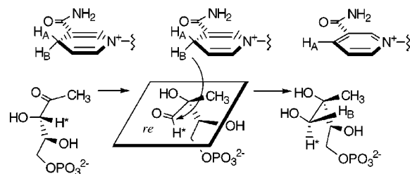
Figure 3. Stereochemical course for DXR-mediated conversion of DXP to MEP.
